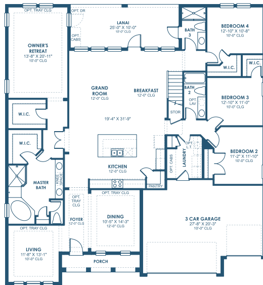
MAIN FLOOR
