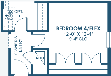
OPT. BEDROOM 4/FLEX
