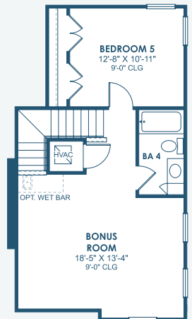
SECOND FLOOR
