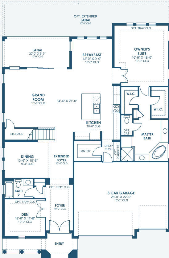
MAIN FLOOR
