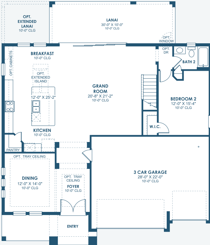
MAIN FLOOR
