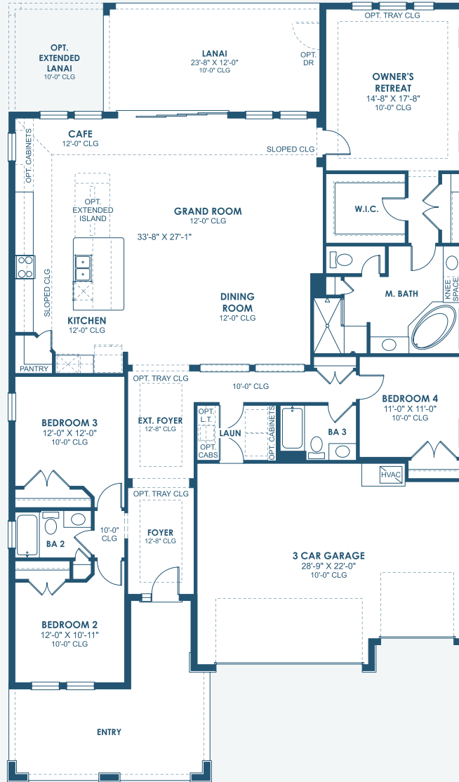
MAIN FLOOR
